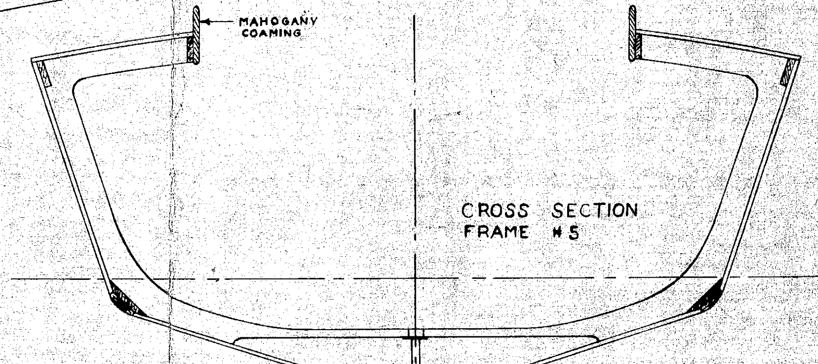
MERCURY CLASS DETAIL PLAN DESIGNED BY ERNEST NUNES
